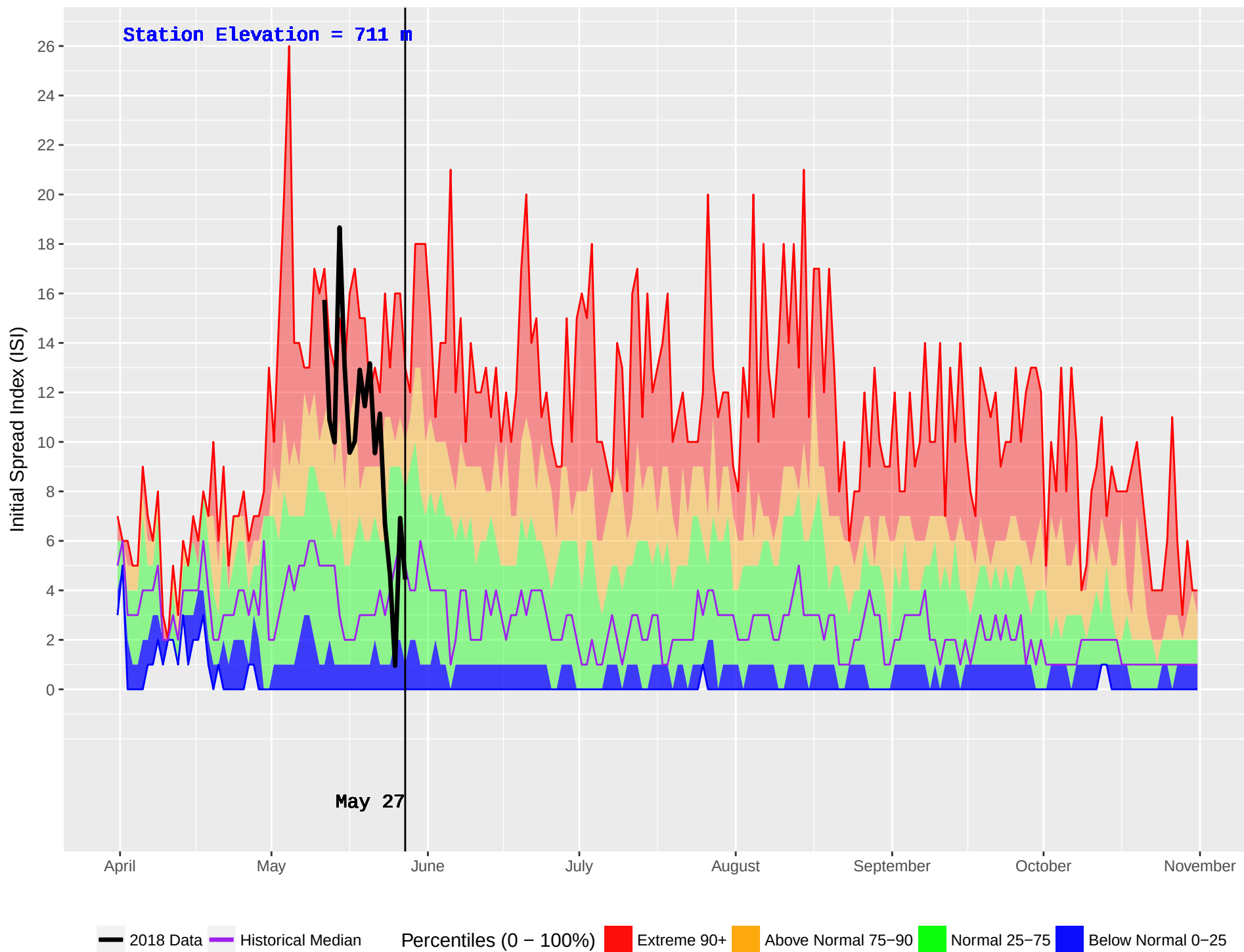
TOAD RIVER (126) : Historical (1981–2016) and Current (2018) Noon Initial Spread Index (ISI)
