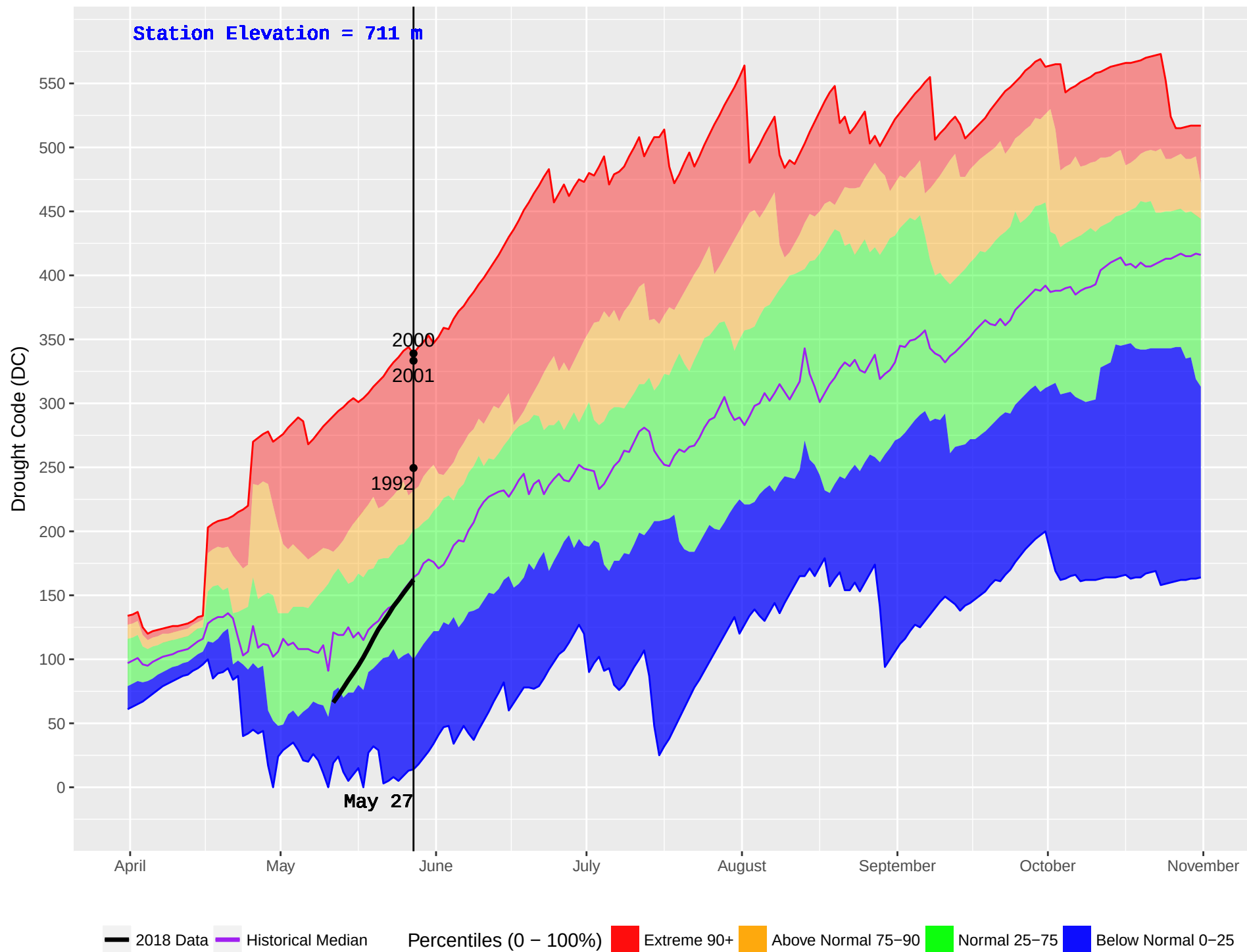
TOAD RIVER (126) : Historical (1981–2016) and Current (2018) Noon Drought Code (DC)
