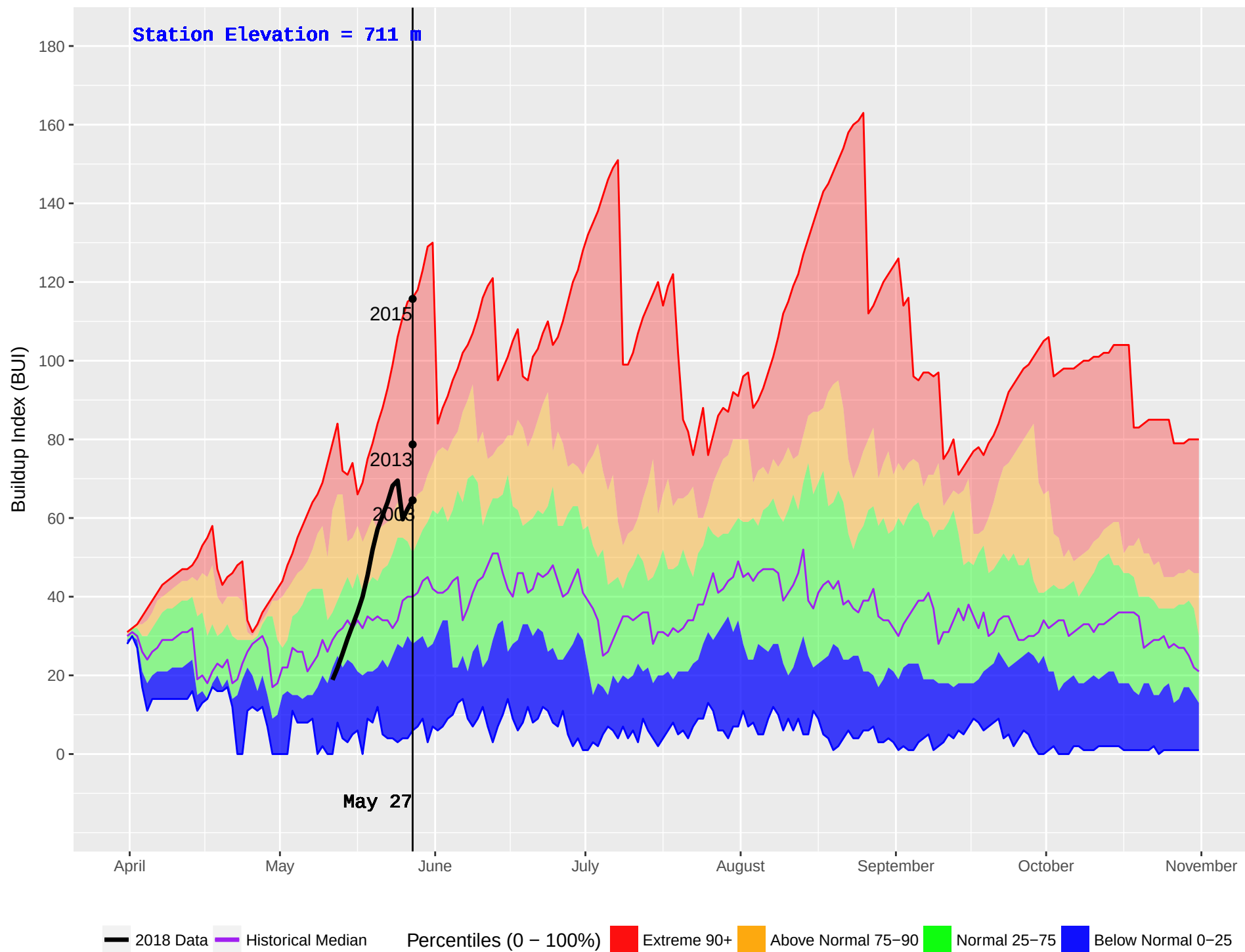
TOAD RIVER (126) : Historical (1981–2016) and Current (2018) Noon Buildup Index (BUI)
