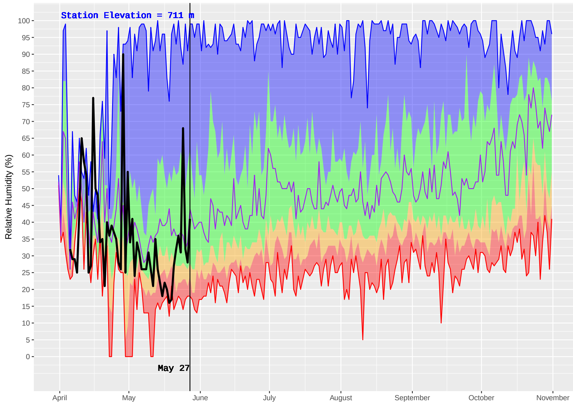
TOAD RIVER (126) : Historical (1981–2016) and Current (2018) Noon Relative Humidity
