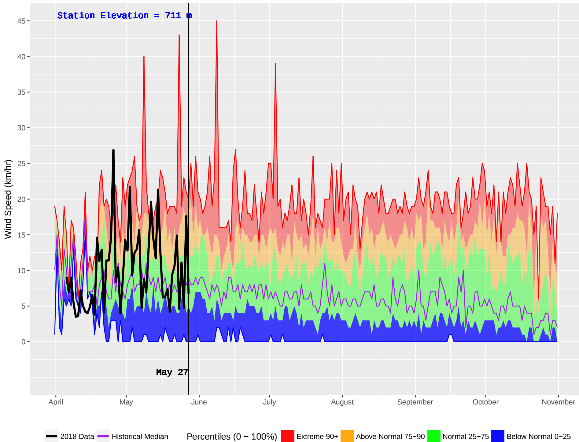
TOAD RIVER (126) : Historical (1981–2016) and Current (2018) Noon Wind Speed
