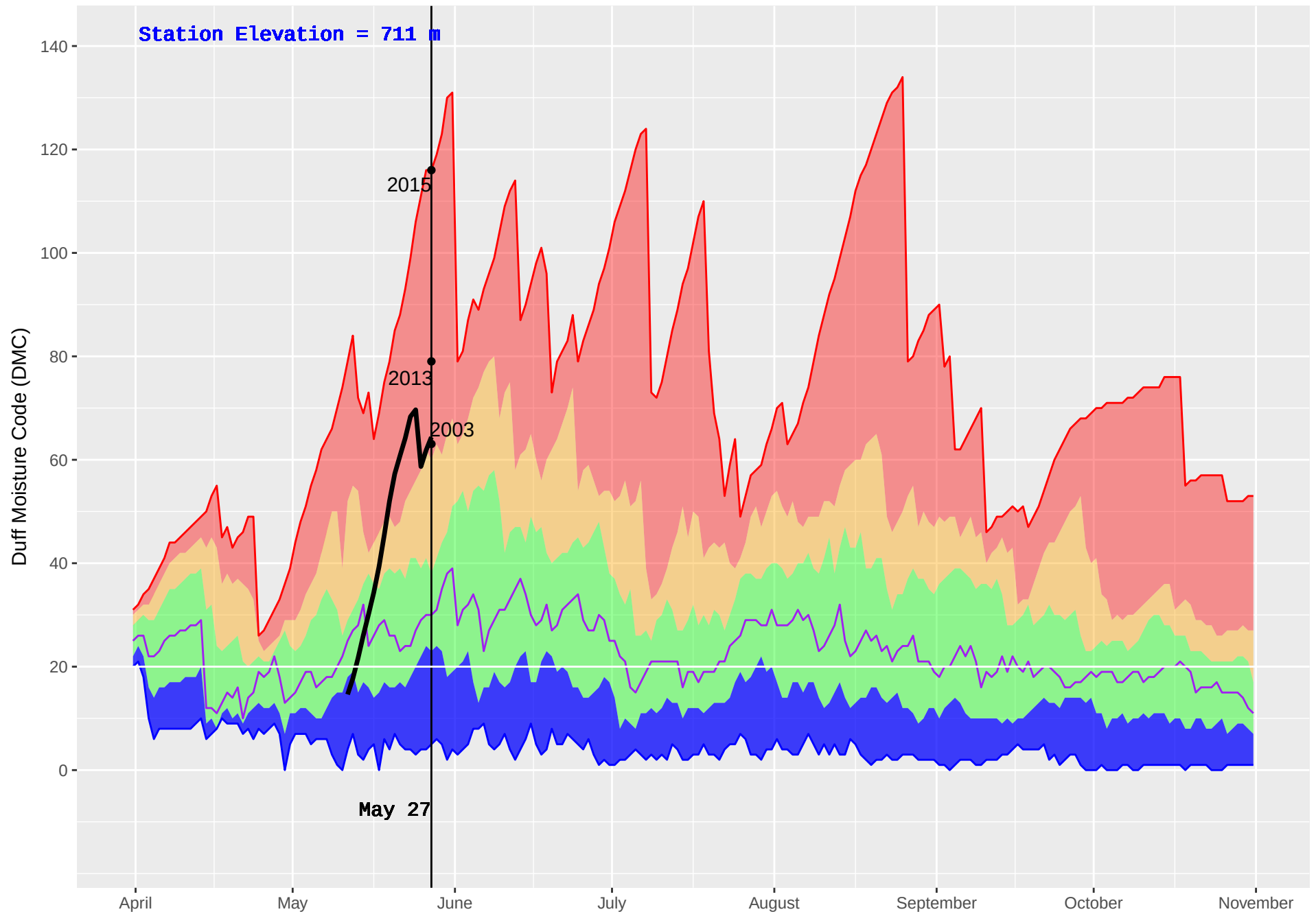
TOAD RIVER (126) : Historical (1981–2016) and Current (2018) Noon Duff Moisture Code (DMC)
