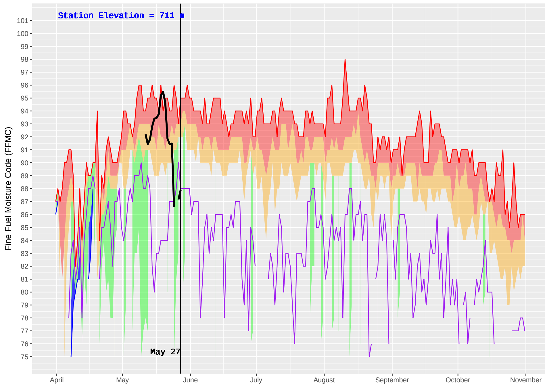
TOAD RIVER (126) : Historical (1981–2016) and Current (2018) Noon Fine Fuel Moisture Code (FFMC)
