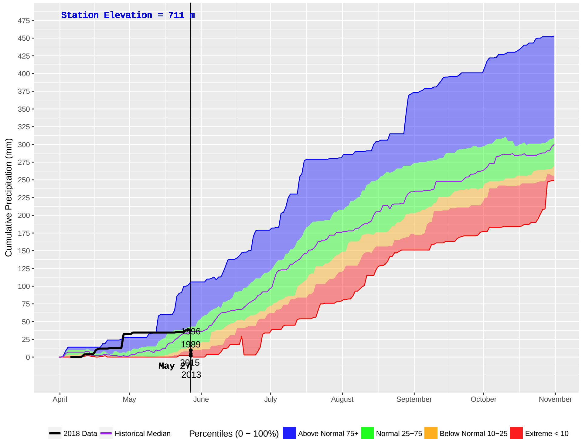
TOAD RIVER (126) : Historical (1981–2016) and Current (2018) Noon Cumulative Precipitation
