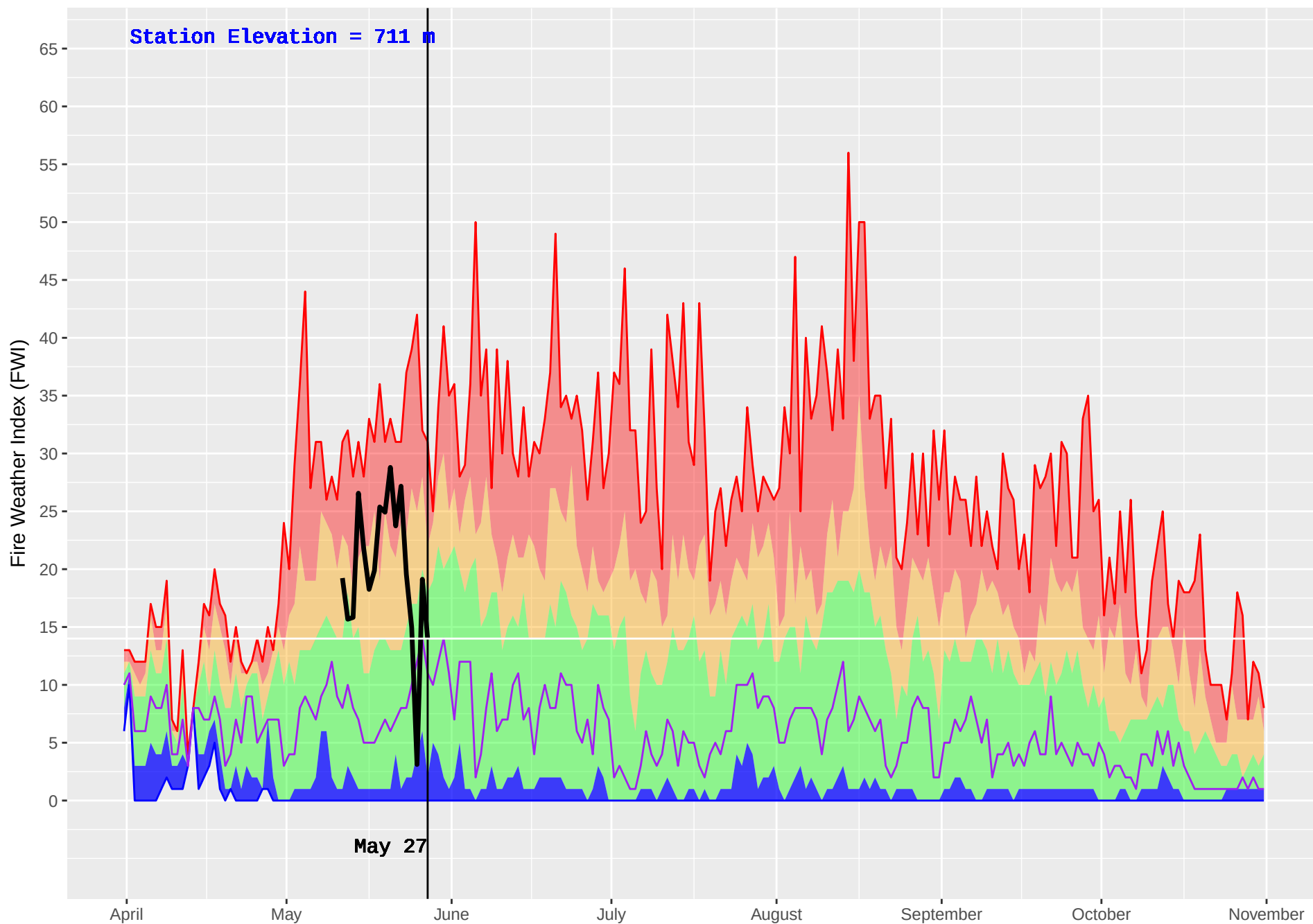
TOAD RIVER (126) : Historical (1981–2016) and Current (2018) Noon Fire Weather Index (FWI)
