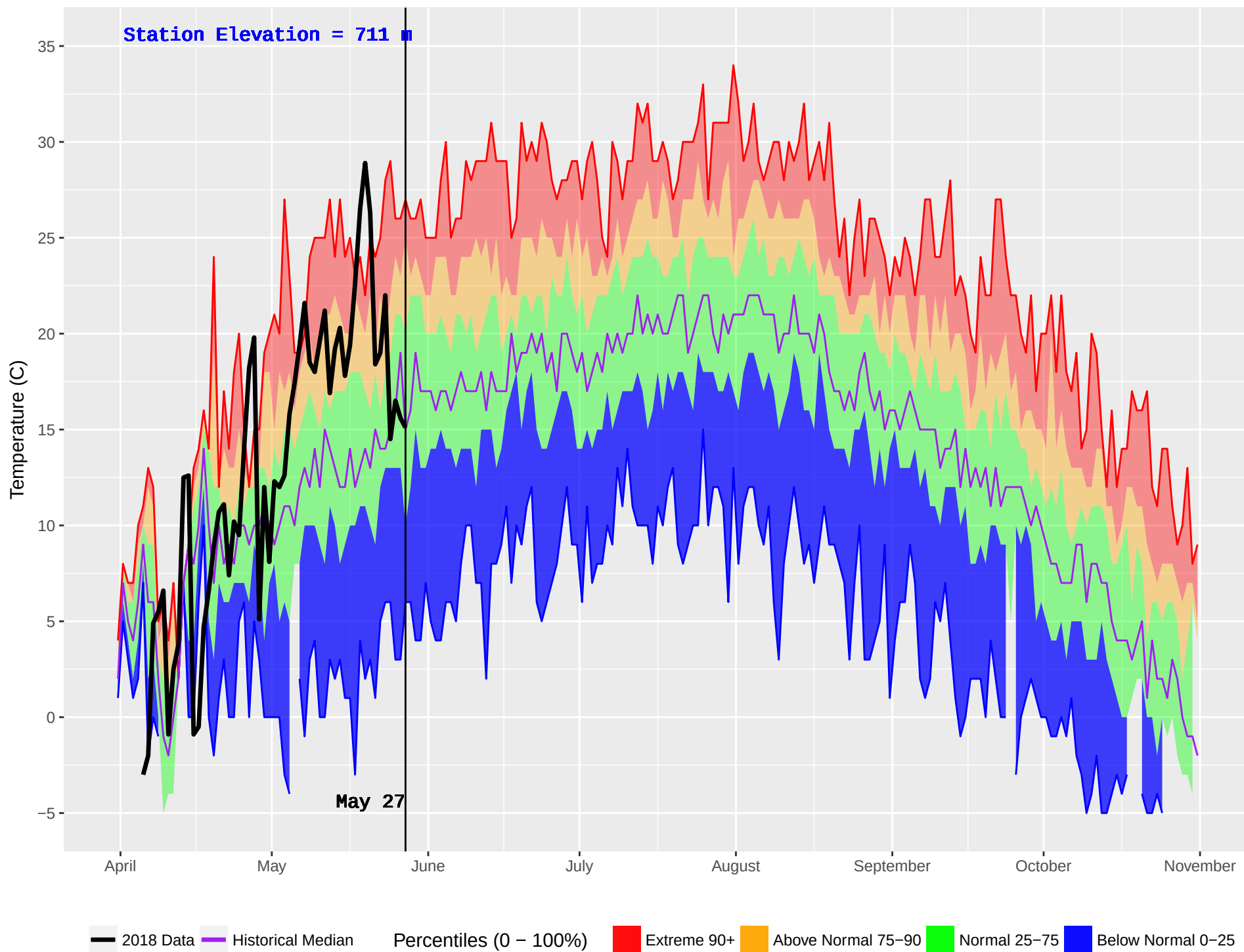
TOAD RIVER (126) : Historical (1981–2016) and Current (2018) Noon Temperature
